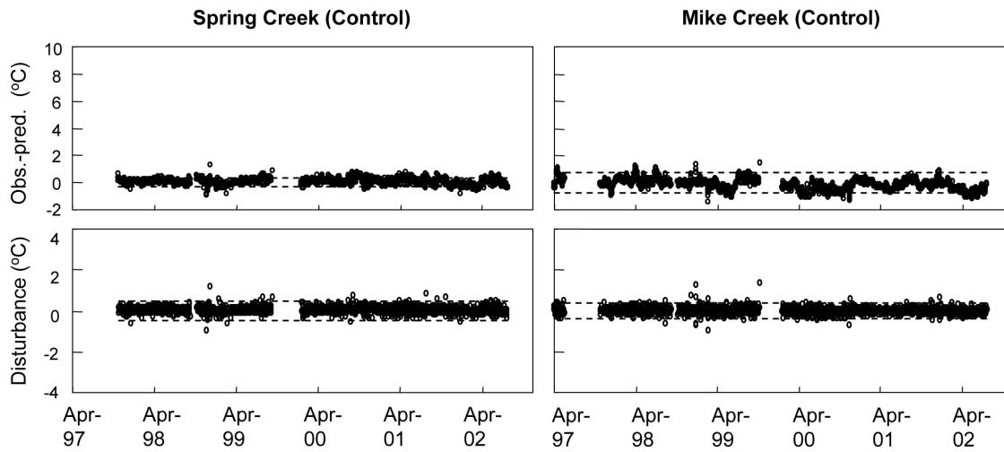
Figure 3. (top) Difference between observed and predicted daily maximum temperature and (bottom) random disturbances in Spring Creek and Mike Creek. Data before 1 April 1999 were used to calibrate the regression model, while data from 1 April 1999 onward were used to test the interannual stability of the model. Dashed horizontal lines in the disturbance plots indicate 95% prediction limits estimated as \pm 1.96 s_u , ( s_u = standard deviation of \hat{u}_t ); dashed horizontal lines in plots of treatment effects show bands of \pm 1.96 s_e (where s_e is the standard error of the residuals from the regression).
