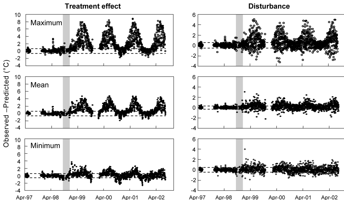
Figure 4. Treatment effects and disturbances for daily maximum, mean, and minimum temperatures for I Creek. See the Figure 3 caption for an explanation of dashed horizontal lines.
