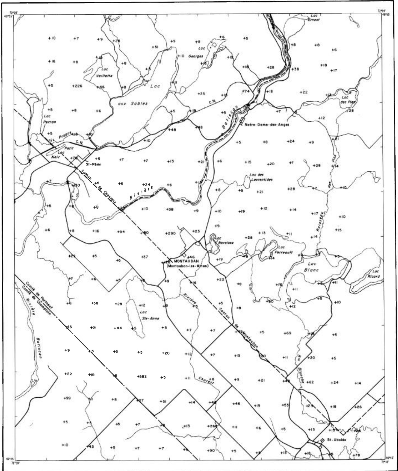
FIGURE 3 - Carte géochimique - As (ppm x 10)
